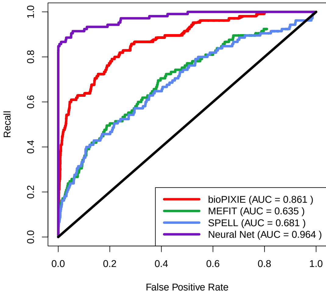
Ensemble Comparison 430x200x1
